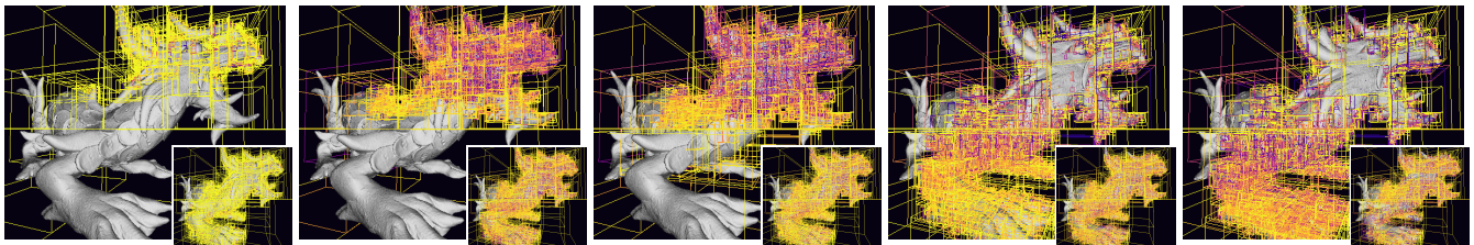
(a) Time series visualization for the Asian Dragon mesh using two different schedulers.
