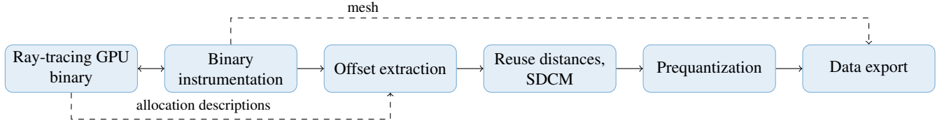
Figure 3: The profiler's internal pipeline. The exported data can subsequently be read by our dashboard.
