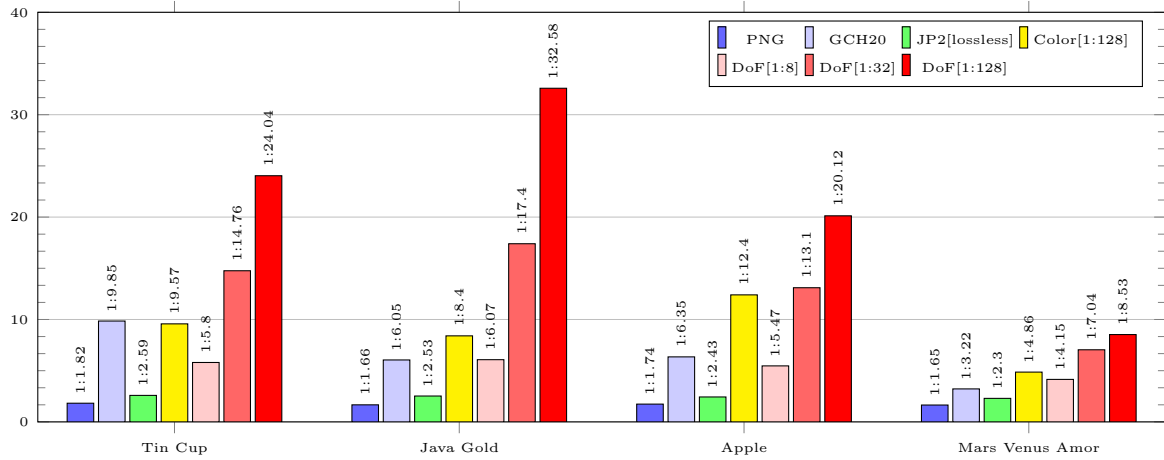
Fig. 6. Compression rate comparison of the PNG algorithm, lossless JPEG2000 and our approach with color and DoF masks. DoF masks are evaluated with lossy background target rates 1:8, 1:32 and 1:128. Color masks are evaluated with lossy background target 1:128 as a comparison.
