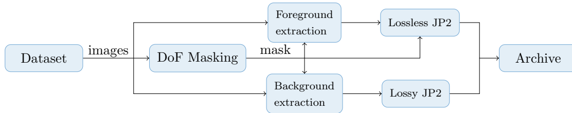
Fig. 1. Overview over the proposed algorithm. First, the images from the dataset are used to create a Depth of Field mask for each image. Then, the mask is used to separate the foreground and the background. The foreground and the mask itself is then encoded using the lossless JPEG2000 algorithm. The background is encoded using the lossy JPEG2000 algorithm. Both compressed images are then saved to the archive.
