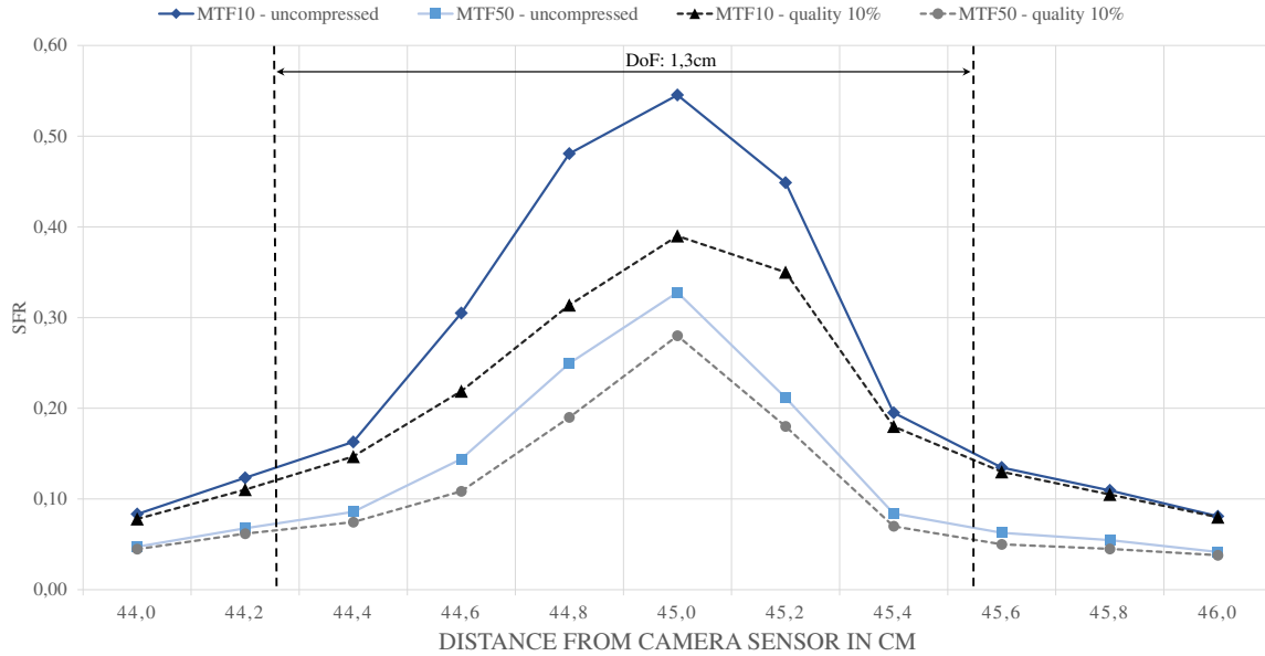
Fig. 4. Evaluated MTF quality metric on a captured SFR target at different distances around a fixed focus distance of 45 cm. For comparison, each image is processed with and without compression.
