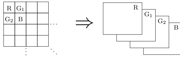
Fig. 2. The Bayer pattern groups four neighboring pixels that can be re-arranged into independent color channels [21].
