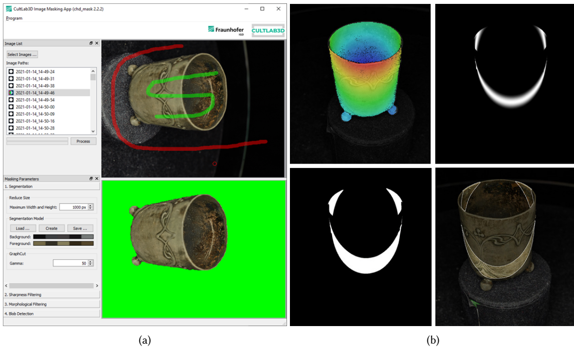
Fig. 3. (a) A graphical user interface for defining initial scribbles for color masking and (b) steps from our fully automatic depth-based masking using depth of field projection.
