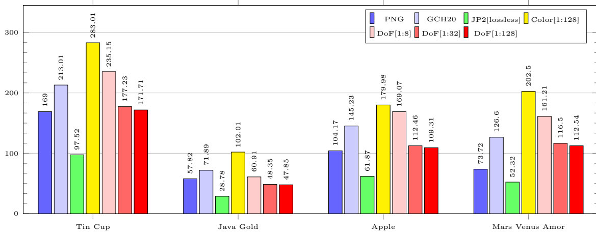
Fig. 7. Run-time performance comparison of the PNG algorithm, lossless JPEG2000 and our approach with color and DoF masks under different background rates. Numbers are in minutes.
