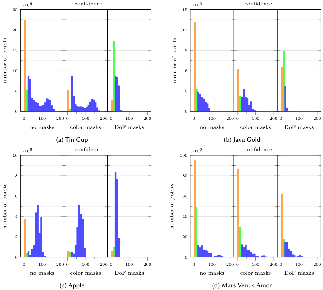
Fig. 9. Histograms showing the confidence values from the point clouds reconstructed from our datasets with no masks applied, with color masks and DoF masks. Orange bars highlight low confidence points with 1 to 10 matches, green bars are points with sufficient confidence with 11 to 20 matches and all other confidence values are marked in blue.
