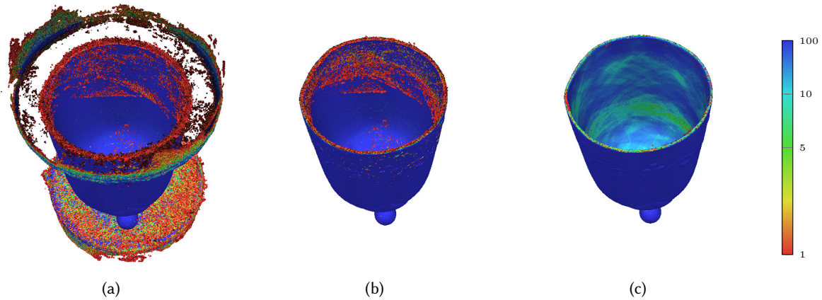
Fig. 8. The confidence point cloud of the Tin Cup dataset reconstructed with different masks. (a) shows the confidence without any masking. The reconstruction of (b) used a color mask and (c) used a DoF mask.
